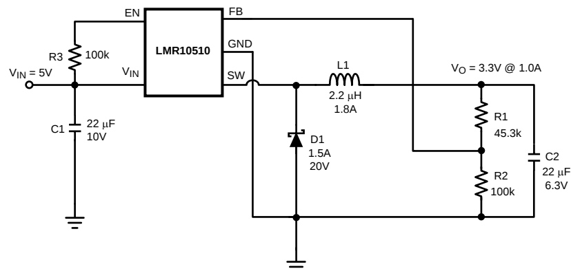
Figure 27. LMR10510X (1.6MHz): V_{IN} = 5V , V_O = 3.3V @ 1.0A
