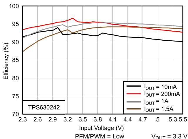
Figure 10. Efficiency vs Input Voltage
