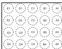
WCSP 20-Pin YFF (TOP VIEW)
