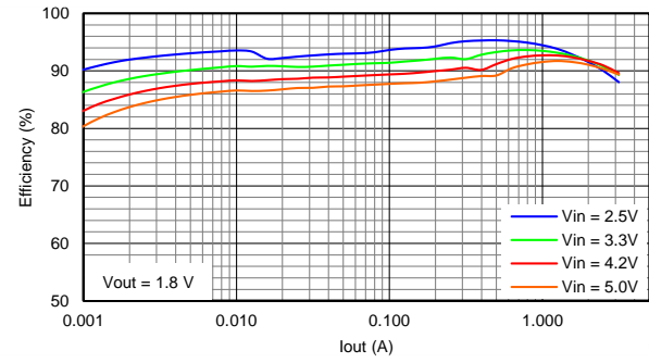
Figure 6. Efficiency
