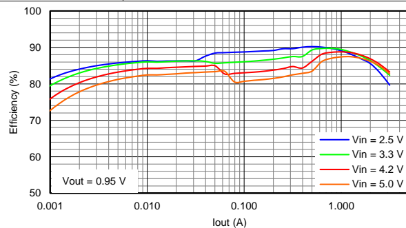
Figure 3. Efficiency
