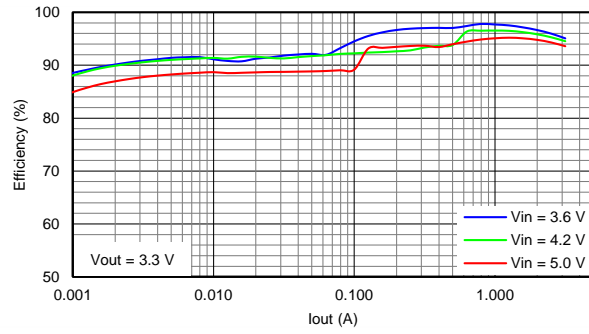
Figure 5. Efficiency
