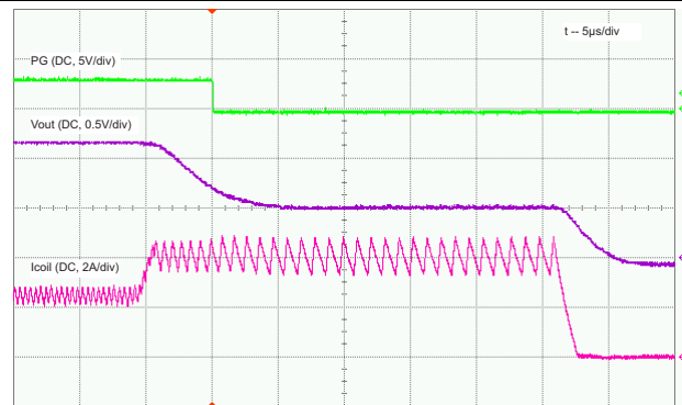
Figure 18. Output Short-Circuit Protection, Load = 0.47 \Omega , Entry
