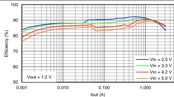
Figure 4. Efficiency
