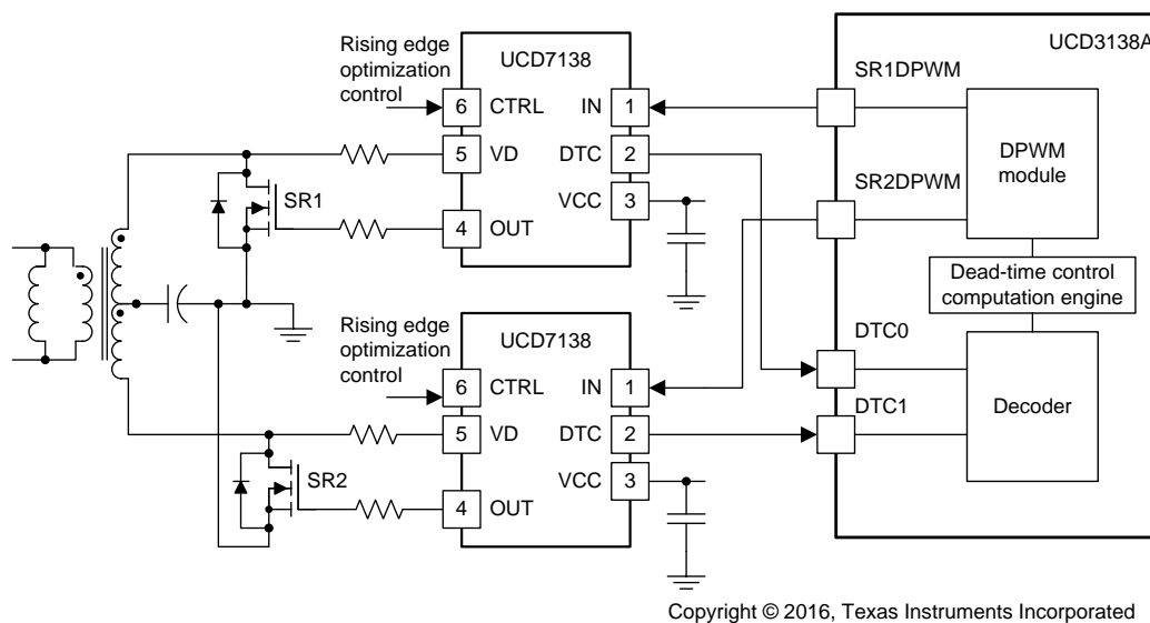
Figure 1-2. Synchronous Rectifier Peripheral Use with Synchronous Rectifier Driver
