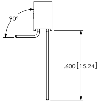
IN PROCESS 2 (LEAD STYLE -01-D,T-RA)
