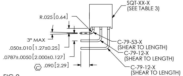
FIG 2 -RA: RIGHT ANGLE (LEAD STYLE -01-D,T)
