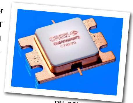
PN: CGHV96050F2 Package Type: 440210
