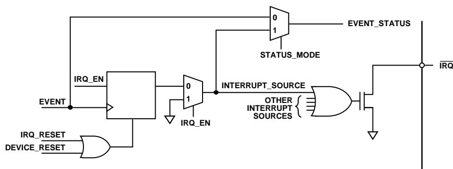
Figure 68. Simplified Schematic of \overline{IRQ} Circuitry
