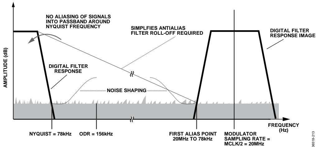
Figure 33. Antialias Example Using the AD7764 in Normal Mode, Decimate x 128 Using MCLK/2 = ICLK = 20 MHz
