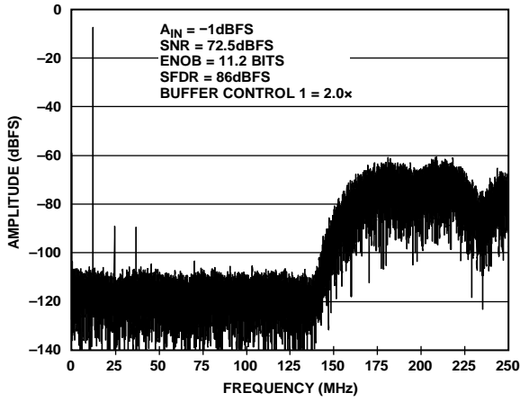
Figure 77. 28% BW Mode, Tuning Word = 0
