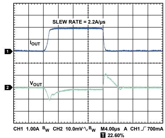
Figure 34. Load Transient Response, I_{LOAD} = 100\text{mA} to 2\text{A} , V_{OUT} = 3.3\text{V} , V_{IN} = 4.0\text{V} , C_{OUT} = 22\mu\text{F} , Channel 1 = I_{OUT} , Channel 2 = V_{OUT}
