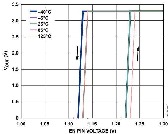
Figure 48. Typical V OUT Response to EN Pin Operation
