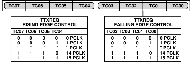
Figure 74. Teletext Control Register
