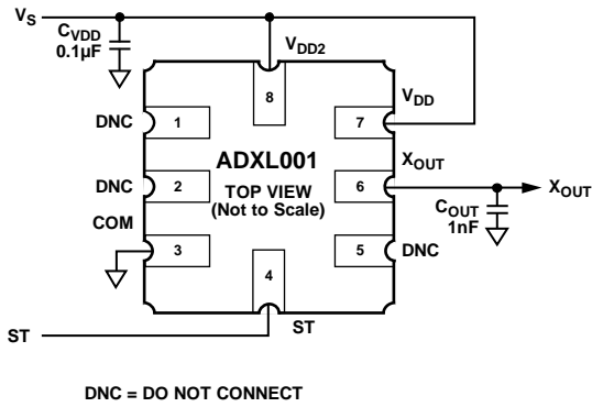
Figure 20. Application Circuit
