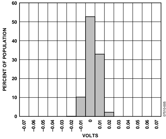
Figure 5. Zero-g Bias Deviation from Ideal
