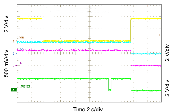
Figure 100. \overline{\text{RESET}} Timing
