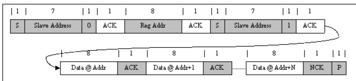
Figure 24. Multi-Read
