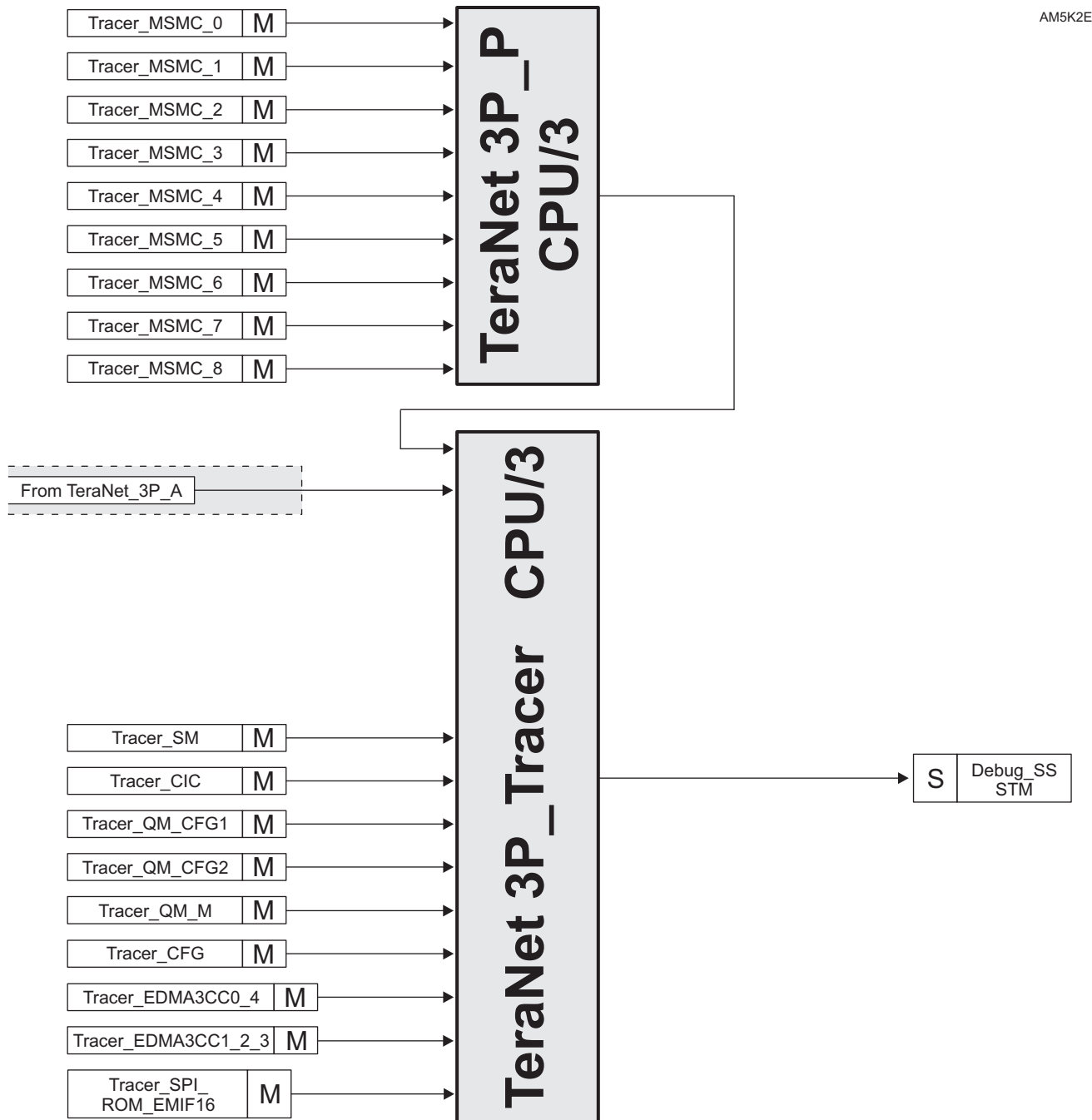
Figure 7-7. TeraNet 3P_Tracer
