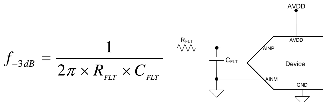
Figure 39. Antialiasing Filter
