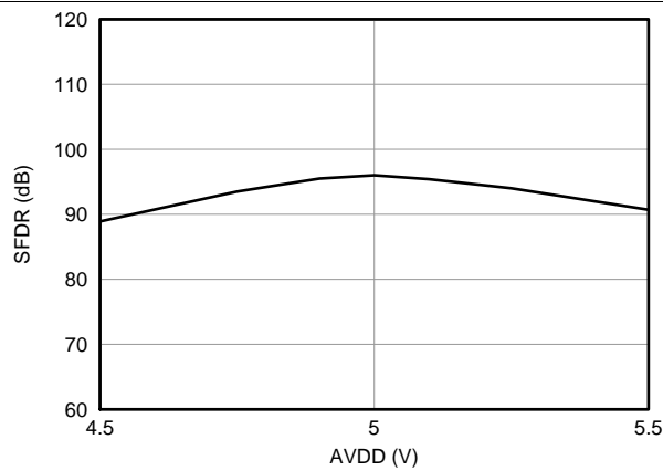
Figure 26. Spurious-Free Dynamic Range vs Analog Supply Voltage
