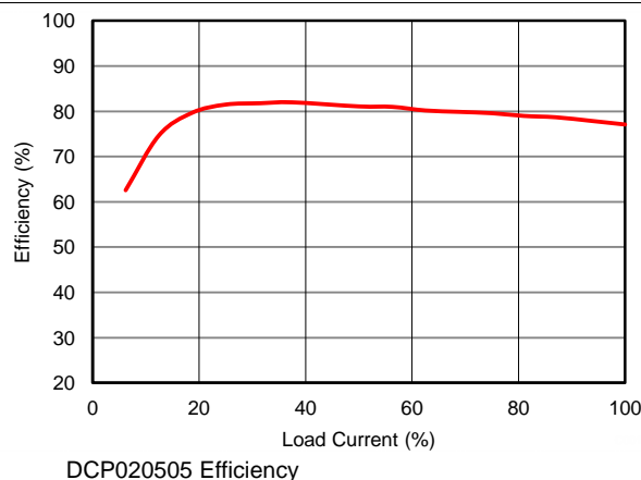
Figure 13. DCP020505 Efficiency
