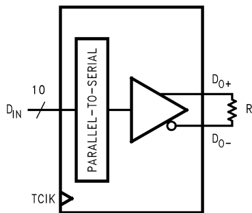
Figure 11. Serializer Delay
