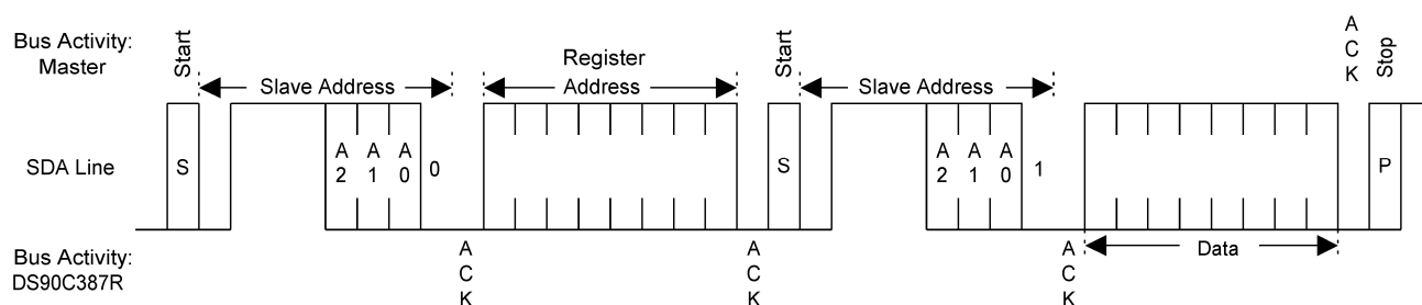
Figure 15. Byte Read
