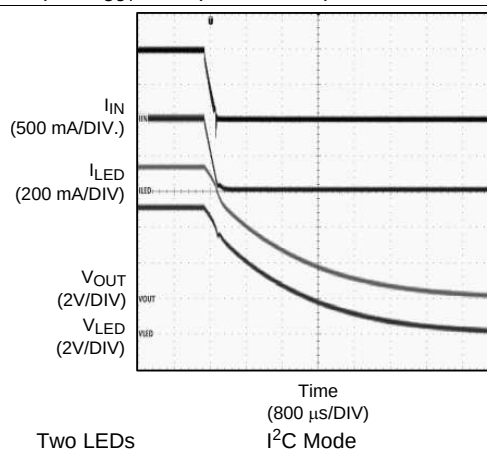
Figure 26. Ramp-Down
