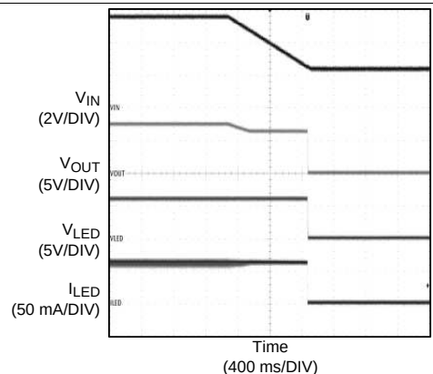
Figure 33. V_{LED} Short to GND Fault
