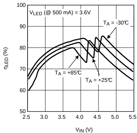
Figure 55. LED Efficiency vs Input Voltage
