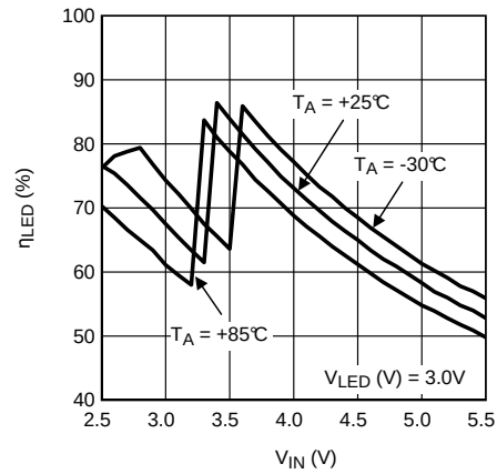
Figure 57. LED Efficiency vs Input Voltage
