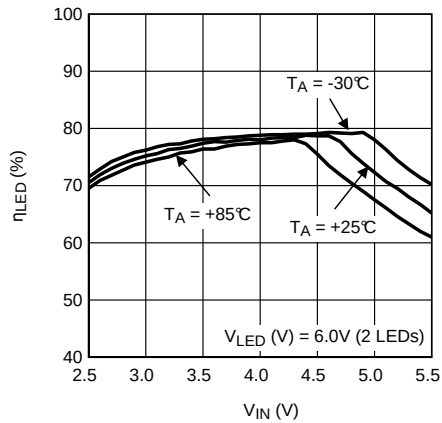
Figure 51. LED Efficiency vs Input Voltage
