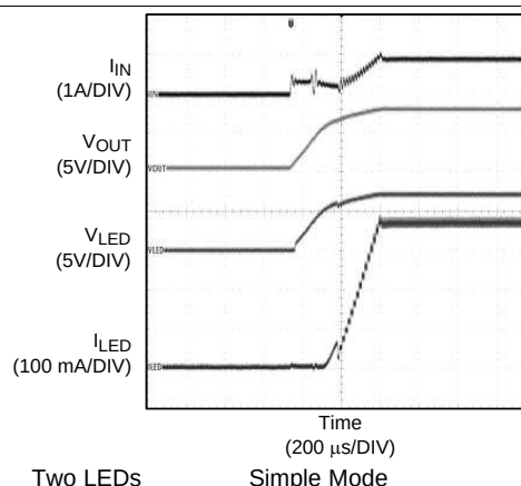
Figure 28. Start-Up
