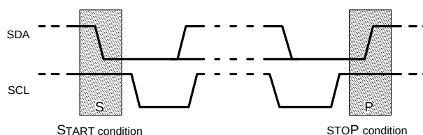
Figure 42. Start and Stop Conditions
