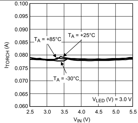
Figure 14. Torch Current vs Input Voltage
