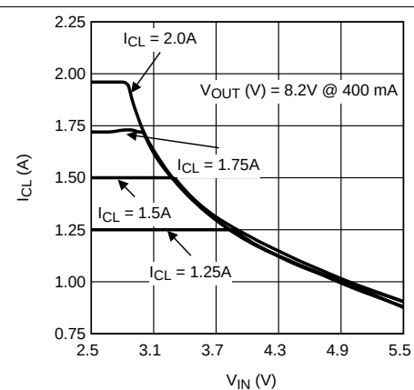
Figure 18. Inductor Current Limit vs Input Voltage
