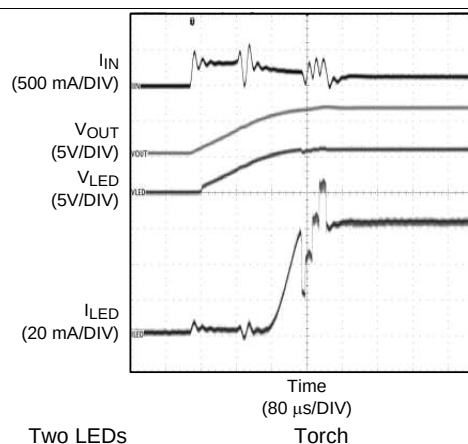
Figure 30. Diode Detect
