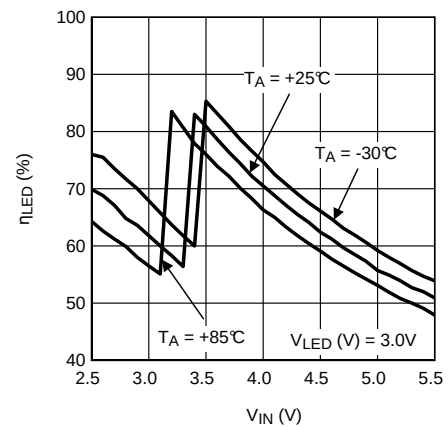
Figure 54. LED Efficiency vs Input Voltage
