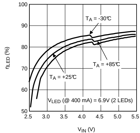
Figure 52. LED Efficiency vs Input Voltage
