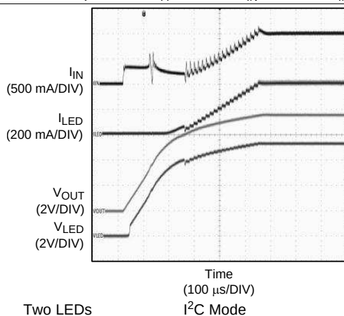
Figure 25. Start-Up
