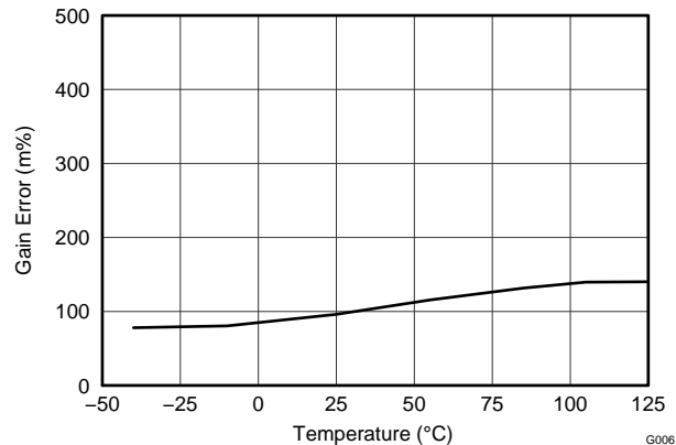
Figure 7. SHUNT INPUT GAIN ERROR vs TEMPERATURE
