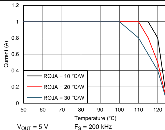
Figure 70. Derating Curve
