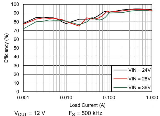
Figure 84. Efficiency
