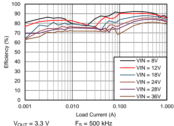
Figure 54. Efficiency
