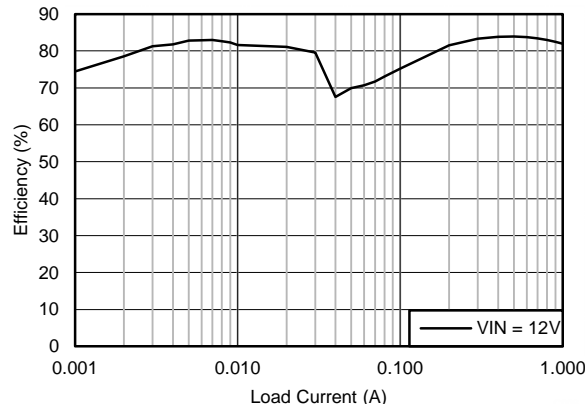
Figure 78. Efficiency
