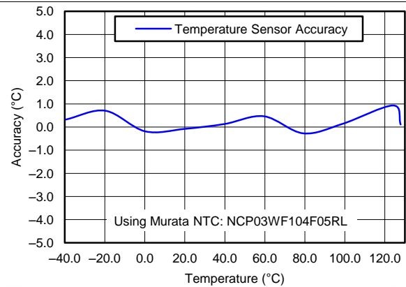
Figure 3. Temperature Accuracy
