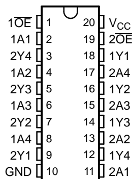
PW PACKAGE (TOP VIEW)
