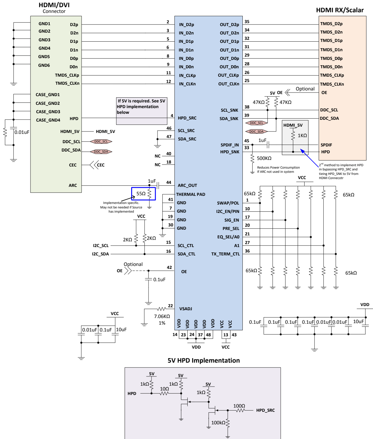
Figure 60. TMD5171 in Sink Side Application, 5 V HPD Implementation
