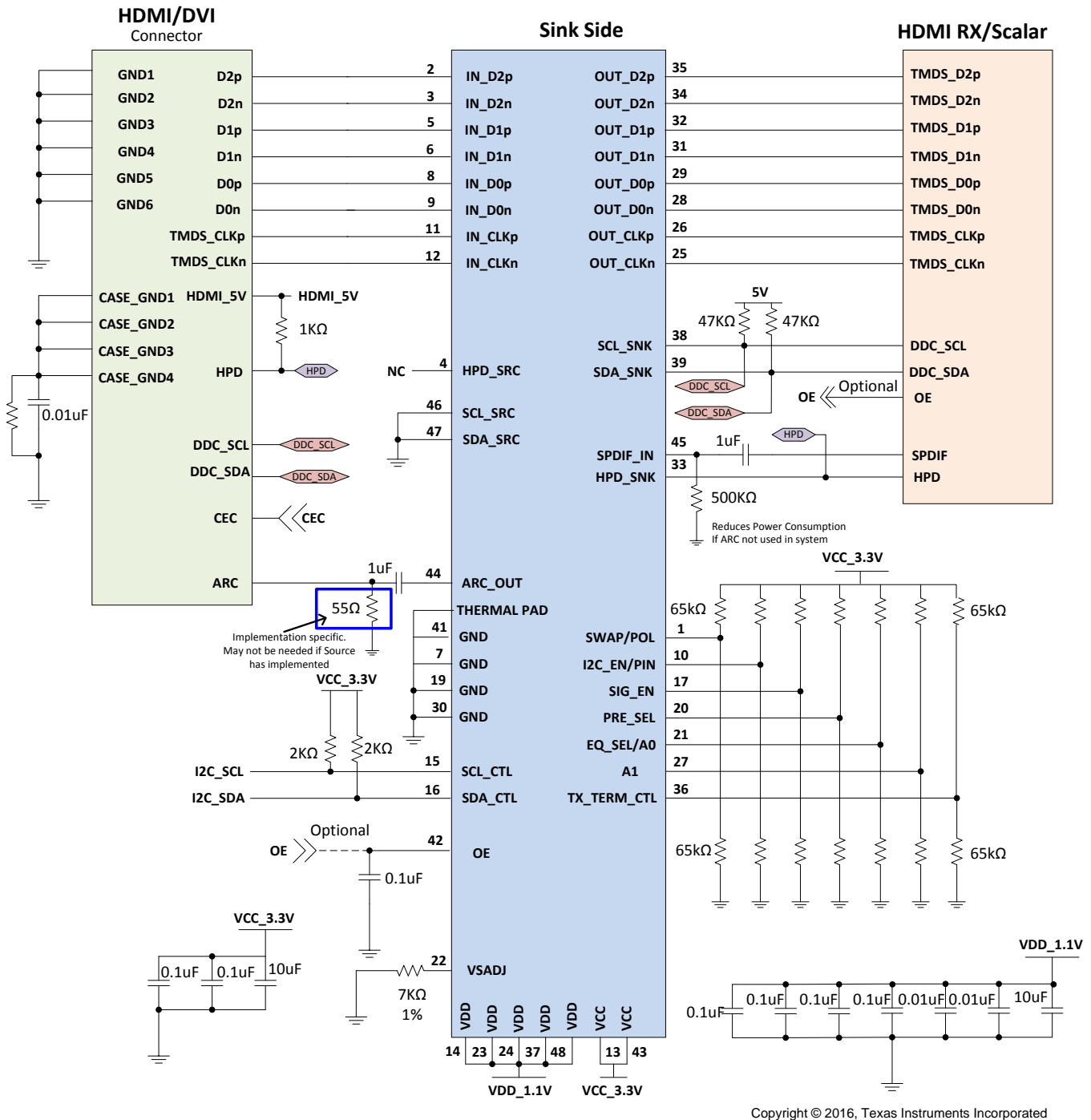
Figure 61. TMD5171 in Sink Side Application
