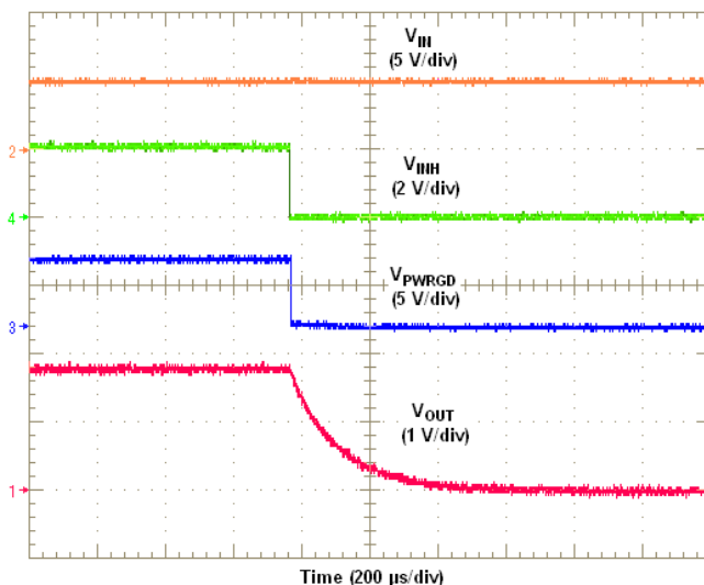
Figure 23. Inhibit Turn-Off
