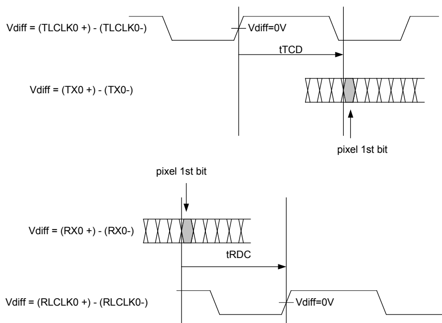
Figure 16. THCV215 and THCV216 Latency
