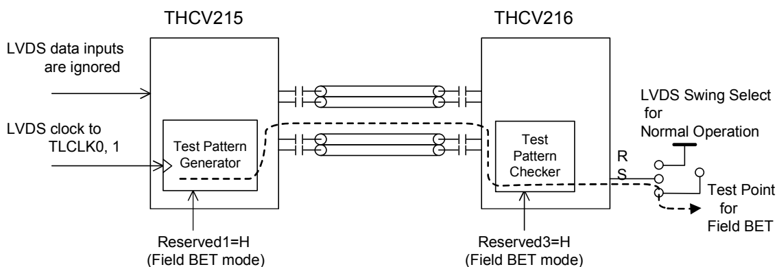
Figure 8. Field BET Configuration
