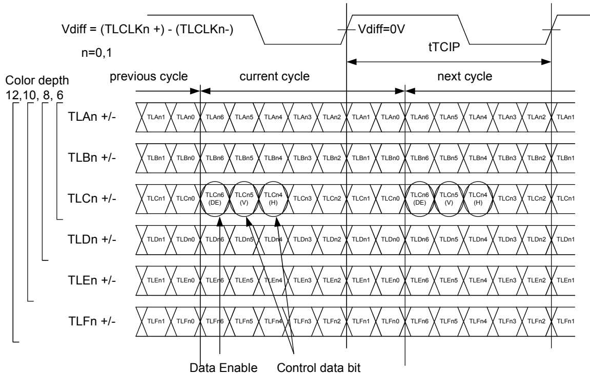
Figure 4. LVDS mapping timing diagram
