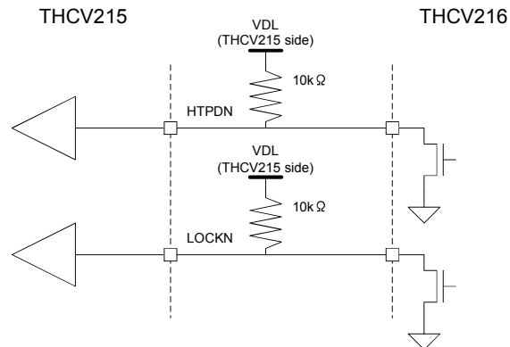
Figure 6. Hot-plug and Lock detect scheme
