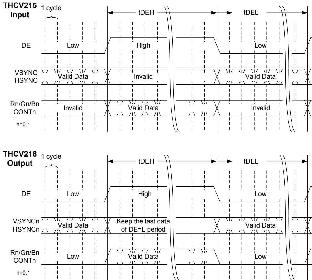
Figure 3. Video and sync data transmission timing diagram
