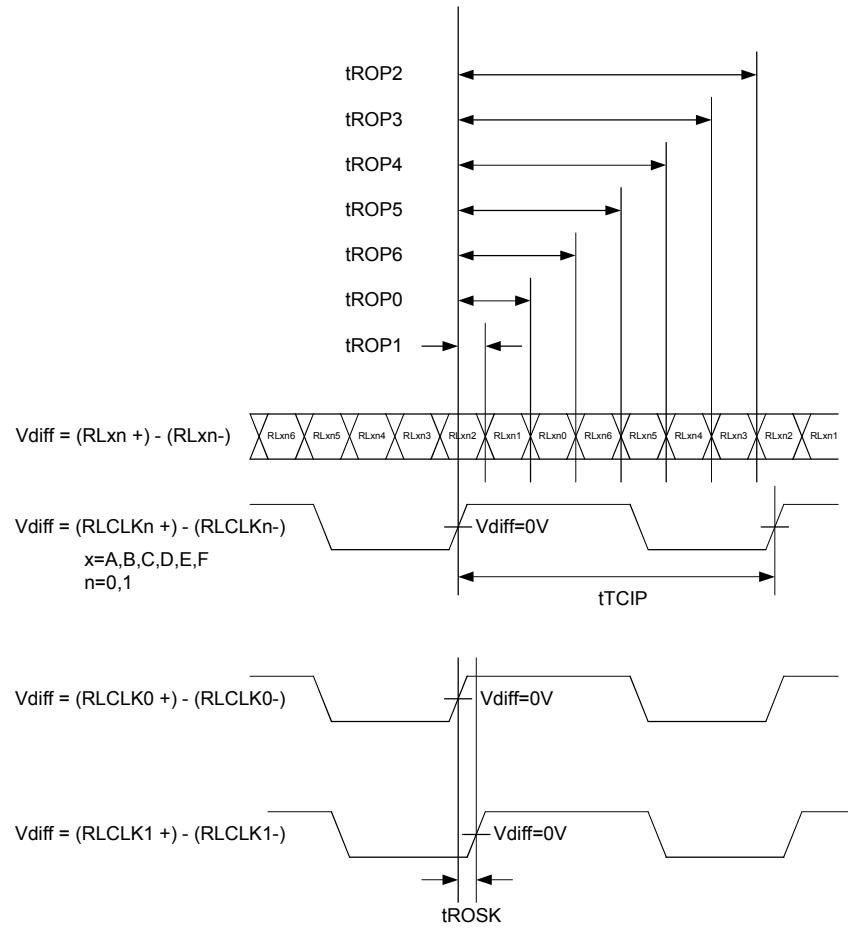
Figure 11. THCV216 LVDS Output Switching Timing Diagrams
