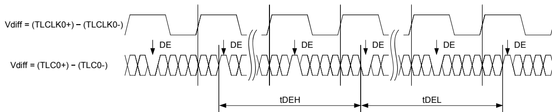
Figure 15. DE period requirement
