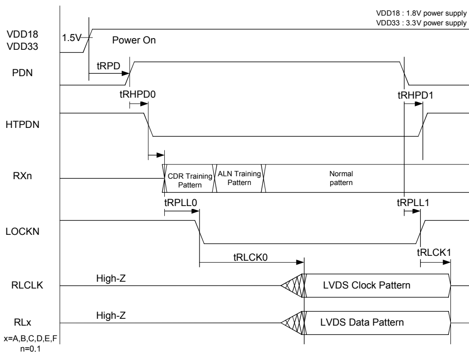
Figure 18. THCV216 Lock/Unlock Sequence
