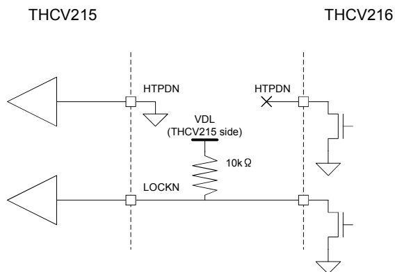
Figure 7. HTPDN is not connected scheme
