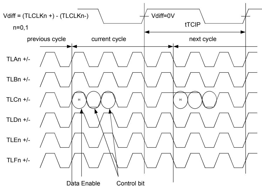
Figure 9. Worst Case Pattern
