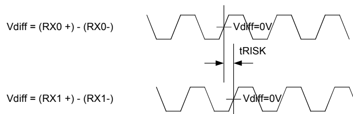
Figure 14. THCV216 CML Input Timing Diagrams
