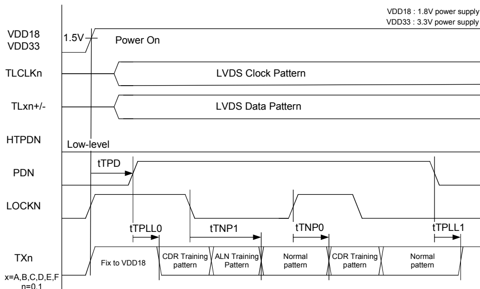
Figure 17. THCV215 Lock/Unlock Sequence
