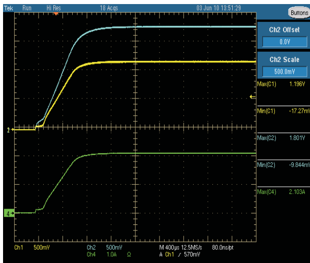
Figure 7. Soft Start for Buck 1 (Yellow Trace) 1.2 V, 3 A and Buck 2 (Blue Trace) 1.8 V, 2 A, V_{IN} = 12\text{ V, } f_{SW} = 500\text{ kHz, } L_O = 4.7\ \mu\text{H,} \text{DCR} = 10\ \text{m}\Omega, C_O = 22\ \mu\text{F}
