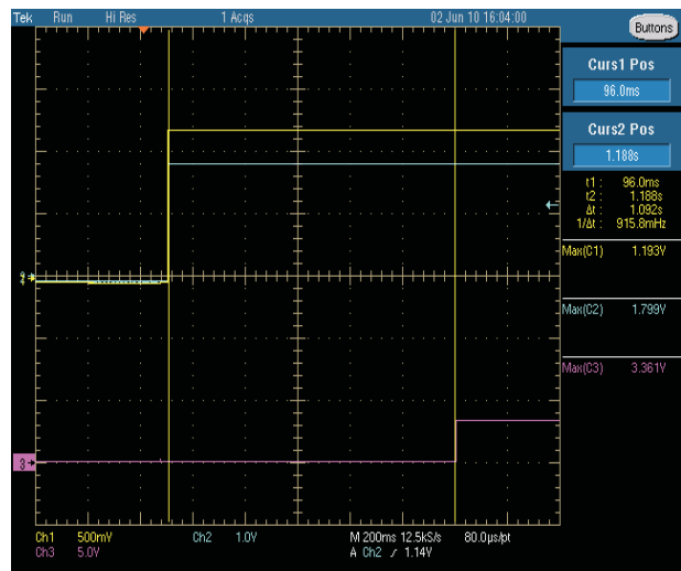
Figure 8. Power Up and PGOOD (From Top to Bottom, Buck2 = 1.8 V, Buck1 = 1.2 V, PGOOD) V_{IN} = 12\text{ V, } f_{SW} = 500\text{ kHz, } L_O = 4.7\ \mu\text{H,} \text{DCR} = 10\ \text{m}\Omega, C_O = 22\ \mu\text{F}
