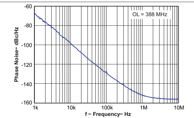
Figure 7. Open Loop VCO Phase Noise
