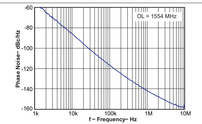
Figure 3. Open Loop VCO Phase Noise
