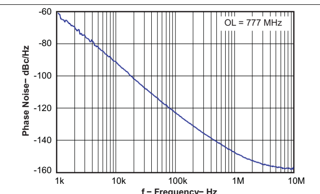
Figure 5. Open Loop VCO Phase Noise
