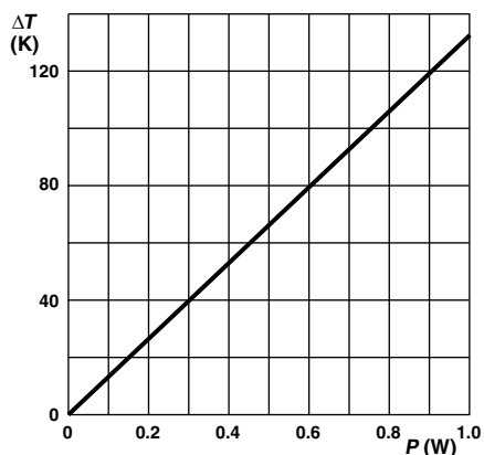
Ø 0.58 mm Cu-leads
