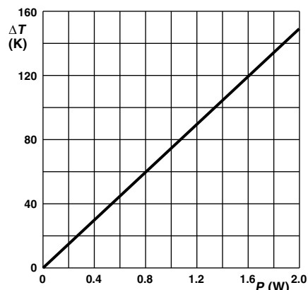
Ø 0.78 mm Cu-leads
