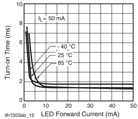
ih1503ab_15 Fig. 16 - Turn-on Time vs. LED Current
