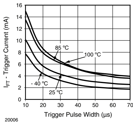
Fig. 11 I_{FT} vs. LED Pulse Width
