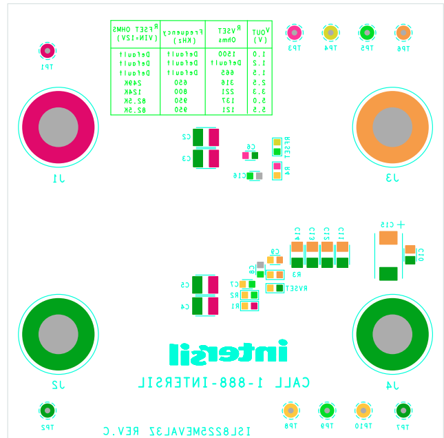
FIGURE 8. BOTTOM COMPONENTS
