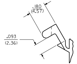
DETAIL 4 .093/(2.36) PREBENT MOUNTING EAR (SCALE 4:1)
