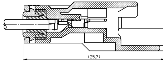
断面A-A (端子装着状態) SECTION A-A (TERM. ASSEMBLY DRAWING)
