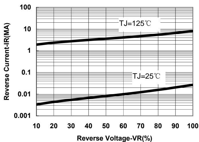
Fig.2-Typical Reverse Characteristics
