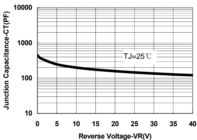
Fig.1-Typical Junction Capacitance
