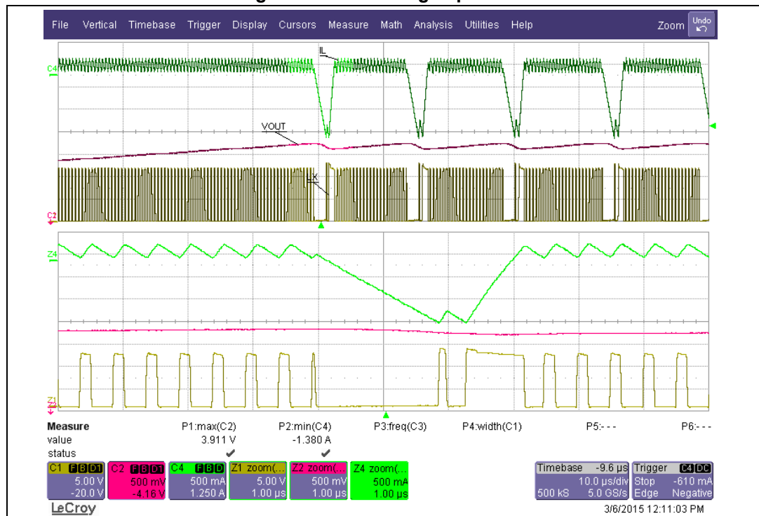
Figure 33. Overvoltage operation
