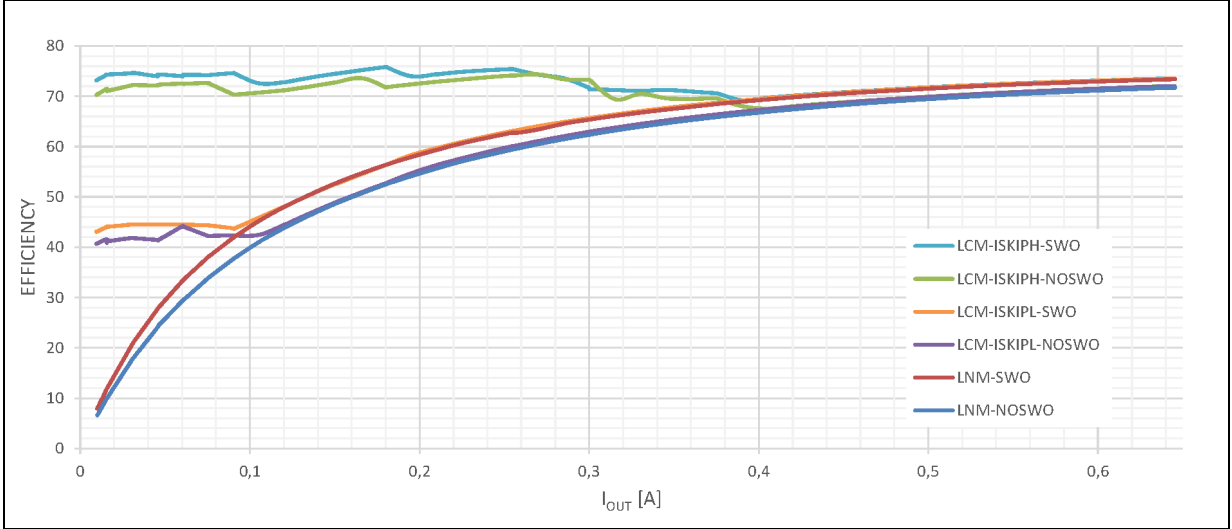
Figure 57. A6985F3V3 efficiency curves: V_{IN} = 13.5\text{ V} - f_{sw} = 2\text{ MHz}
