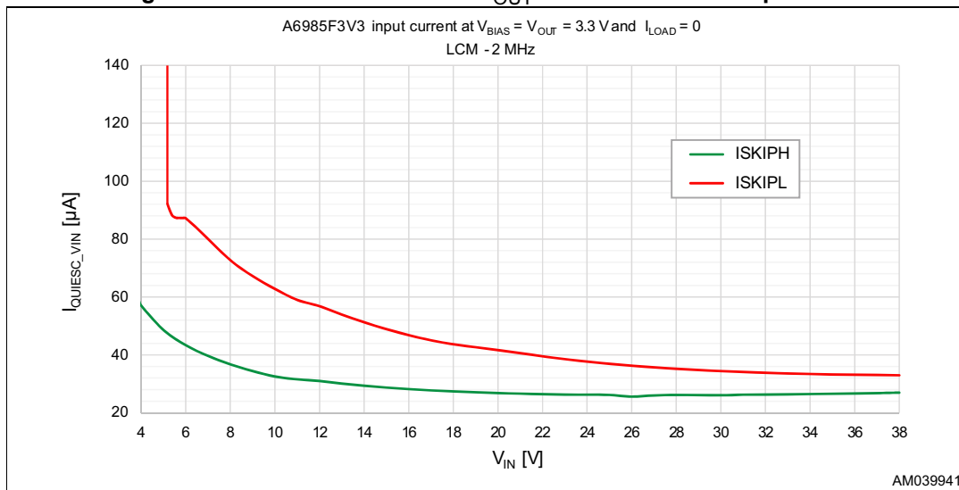
Figure 24. Quiescent current at V_{OUT} = 3.3\text{ V} and zero output load
