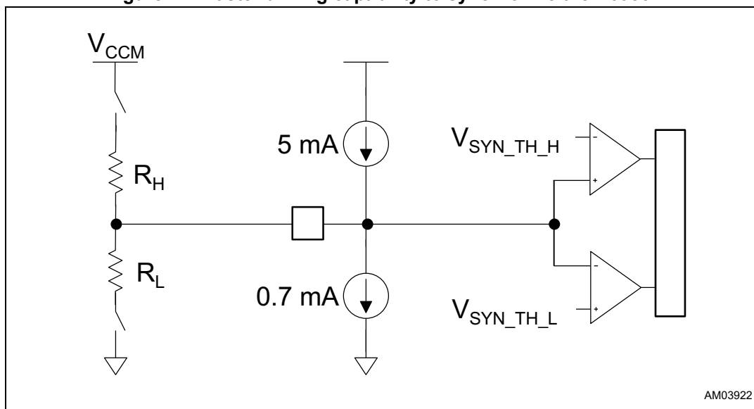
Figure 47. Master driving capability to synchronize the A6985F
