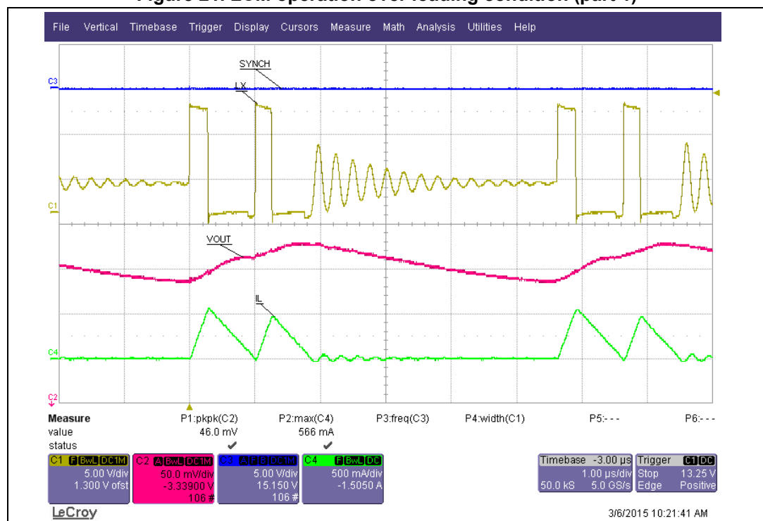
Figure 21. LCM operation over loading condition (part 1)
