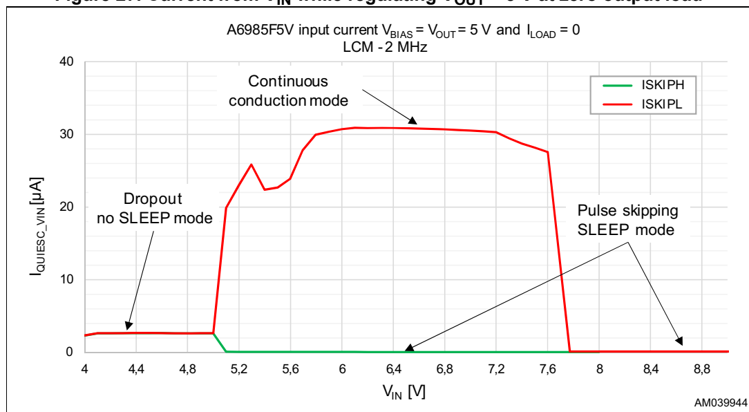
Figure 27. Current from V_{IN} while regulating V_{OUT} = 5 V at zero output load
