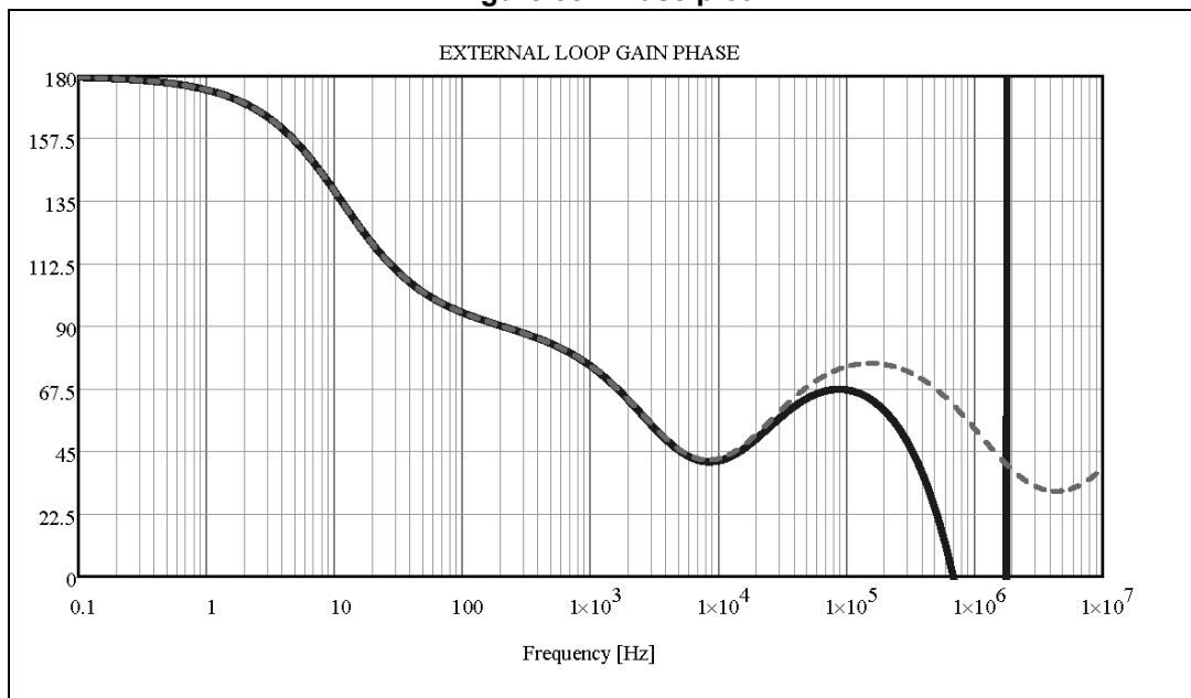
Figure 38. Phase plot
