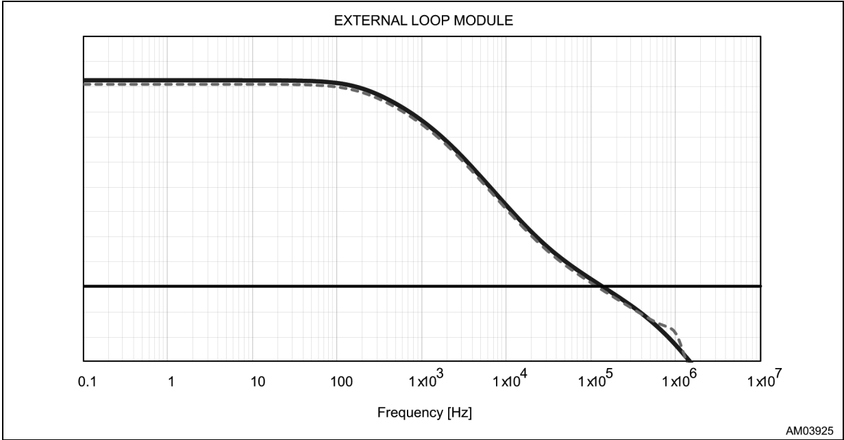
Figure 55. Magnitude Bode's plot of A6985F ( V_{OUT} = 6\text{ V} ) evaluation board
