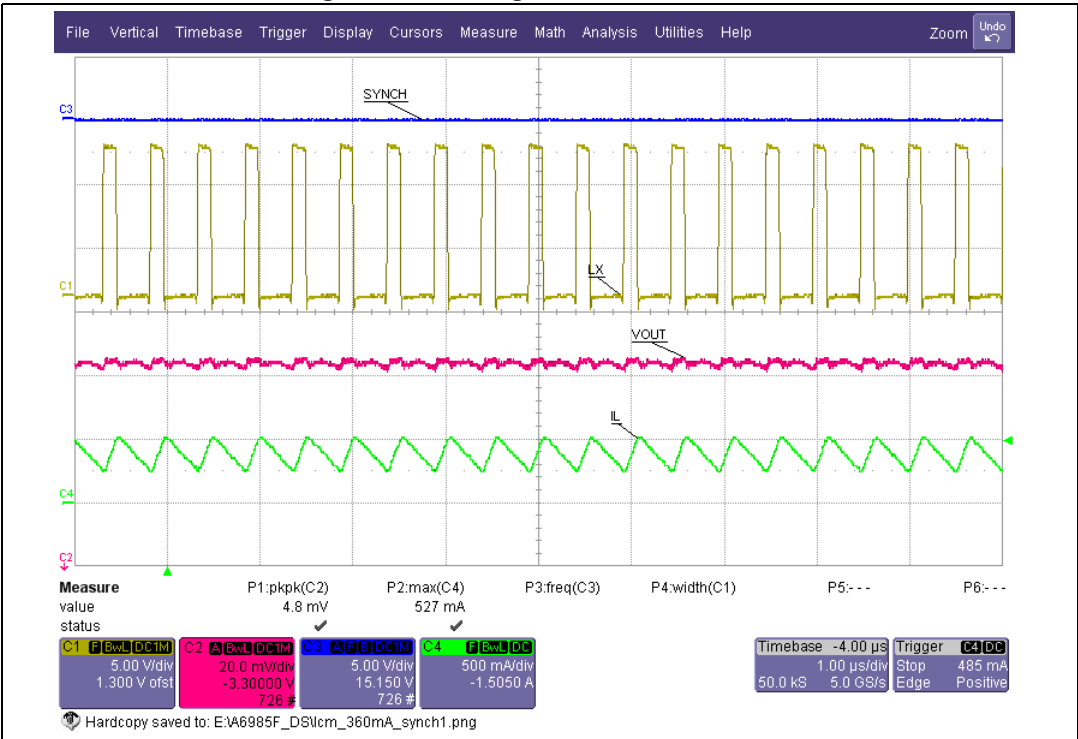
Figure 23. The regulator works in CCM
