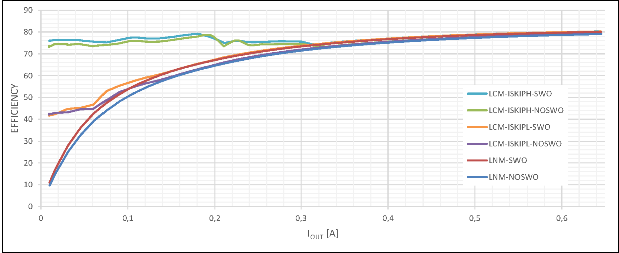
Figure 61. A6985F5V efficiency curves: V_{IN} = 13.5\text{ V} - f_{sw} = 2\text{ MHz}
