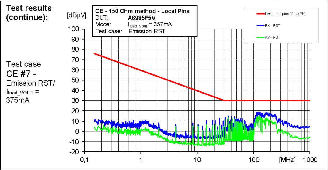
Figure 70. CE 150R at RST test point (see Figure 65 ) at 75% I_{LOAD}
