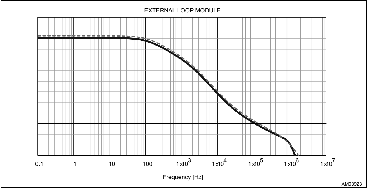
Figure 53. Magnitude Bode's plot of A6985F5V evaluation board
