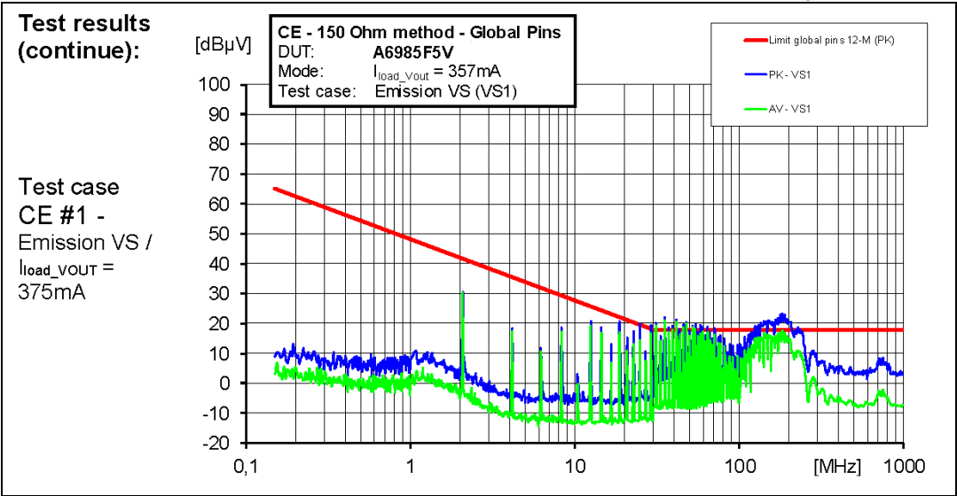
Figure 66. CE 150R at VS1 test point (see Figure 65 ) at 75% I_{LOAD}
