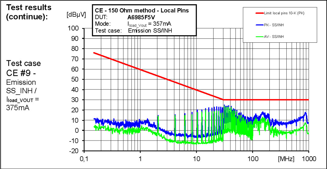
Figure 72. CE 150R at SS/INH test point (see Figure 65 on page 73 ) at 75% I LOAD
