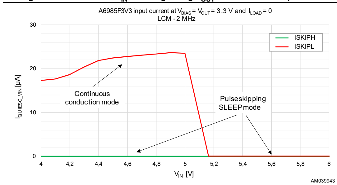
Figure 26. Current from V_{IN} while regulating V_{OUT} = 3.3 V at zero output load
