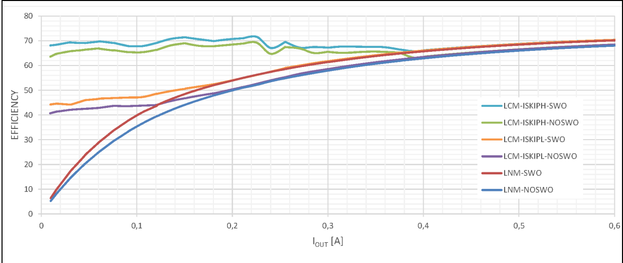
Figure 63. A6985F5V efficiency curves: V_{IN} = 24\text{ V} - f_{sw} = 2\text{ MHz}
