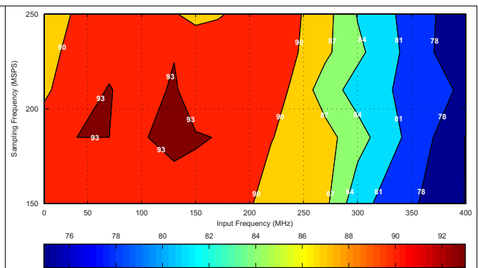
Figure 34. Spurious-Free Dynamic Range (6-dB Gain)
