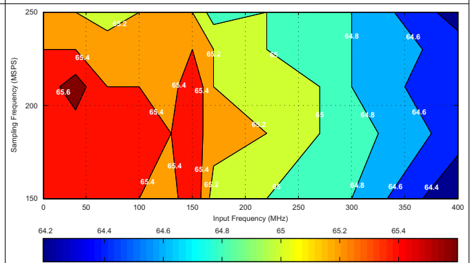
Figure 36. Signal-to-Noise Ratio (6-dB Gain)
