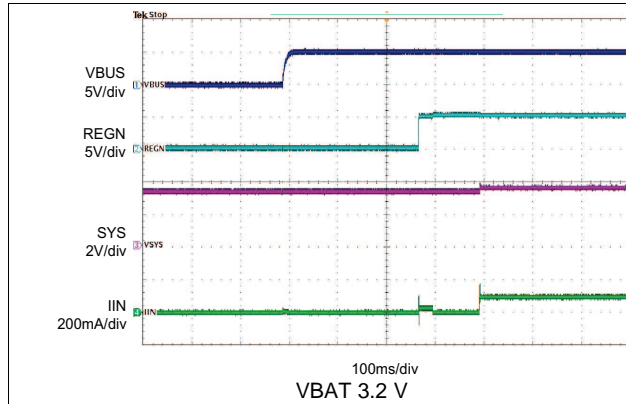
Figure 40. bq24190 Power Up from USB100 mA
