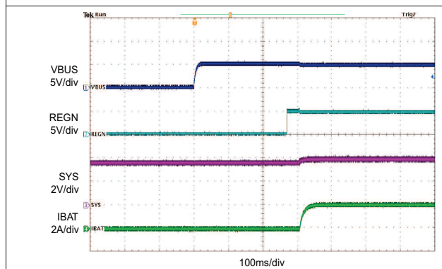
Figure 40. bq24190 Power Up from USB100 mA
