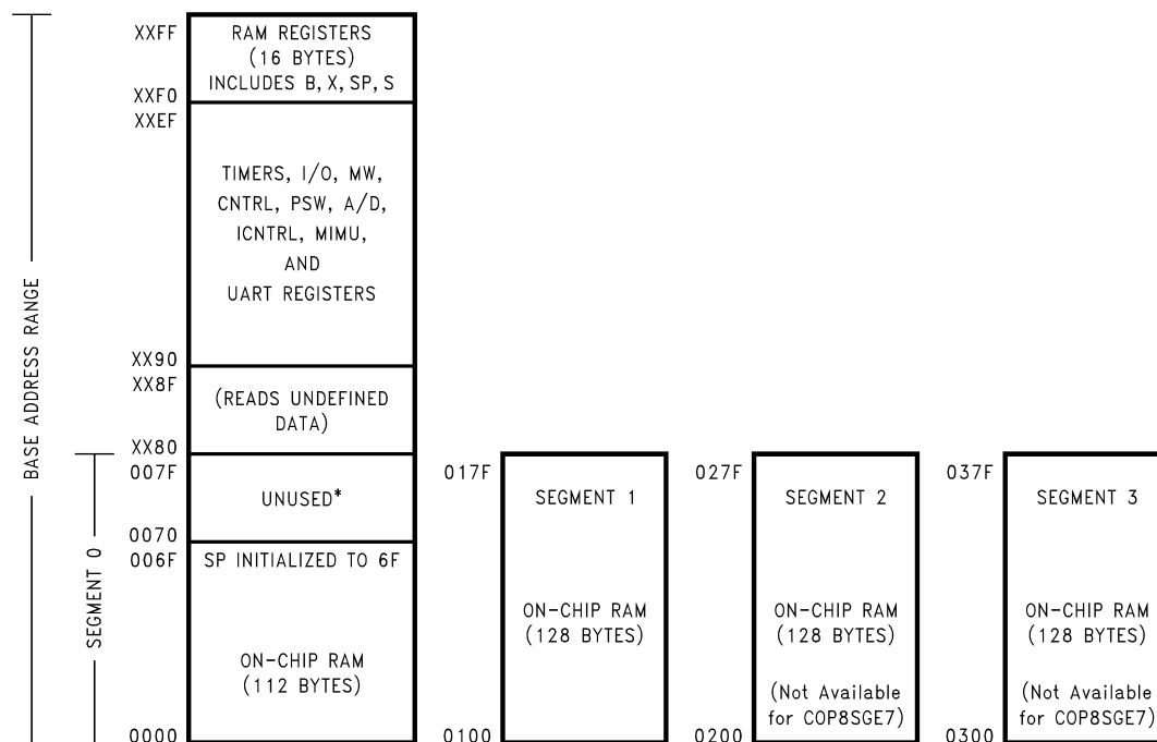
Figure 16. RAM Organization
