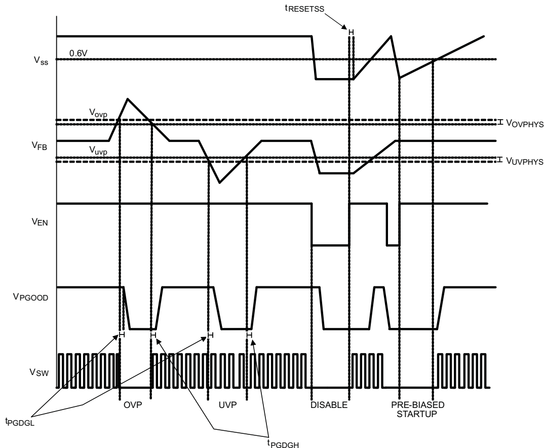
Figure 26. PGOOD Conditions
