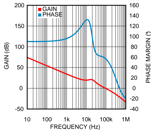
Figure 35. Loop Response
