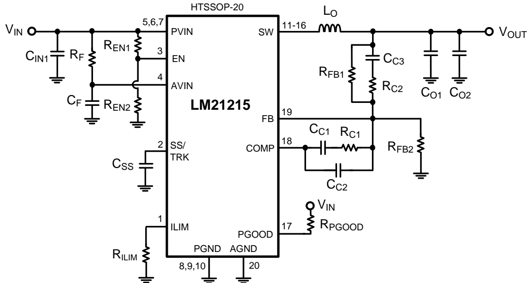
Figure 40. Typical Application Schematic 2
