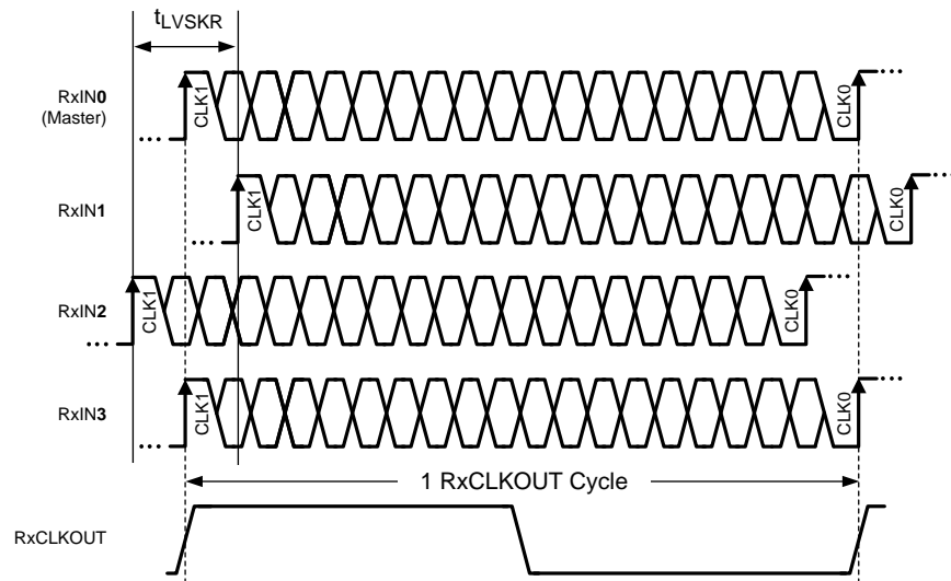
Figure 17. LVDS Deserializer Input Skew
