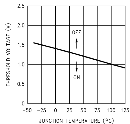
Figure 12. \overline{ON} /OFF Threshold Voltage
