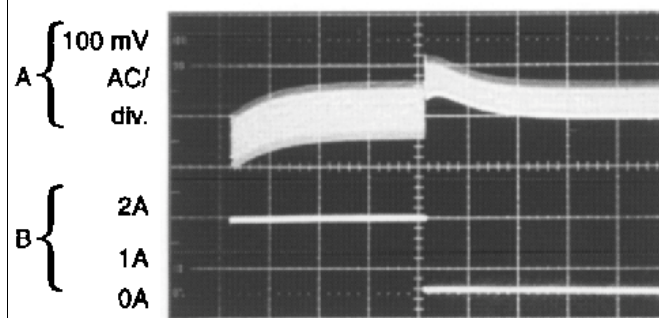
Figure 16. Horizontal Time Base: 2 \mu s /div
