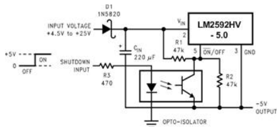
Figure 26. Inverting Regulator Ground Referenced Shutdown Using Opto-isolator Device
