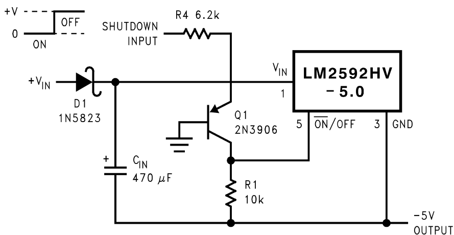
Figure 25. Inverting Regulator Ground Referenced Shutdown
