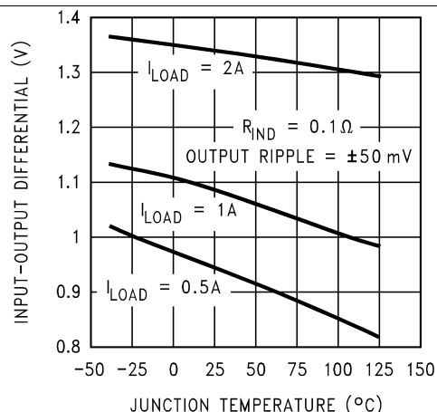
Figure 6. Dropout Voltage
