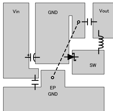
Figure 25. Example PCB Layout
