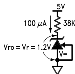
Figure 55. 1.2V Reference
