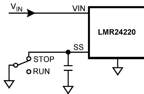
Figure 21. Alternate Shutdown Implementation
