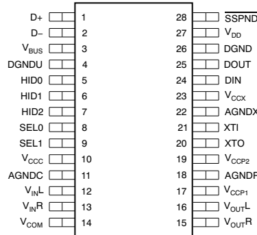
Pin Functions
