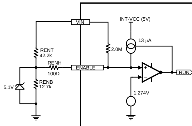
Figure 51. Enable Input Detail
