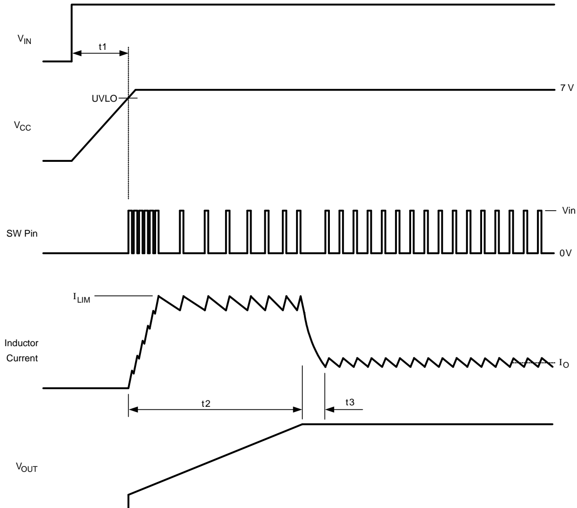
Figure 10. Startup Sequence
